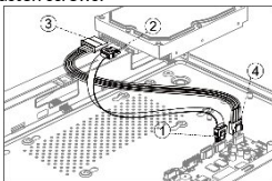
Figure 2-2 Connect Cable
