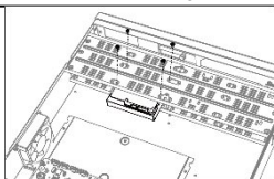
Figure 2-5 Fix HDD
