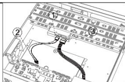
Figure 2-6 Connect Cable
